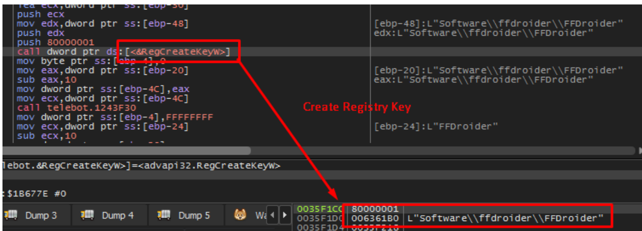
Figure 8: Creates a registry key named “FFDroider”
