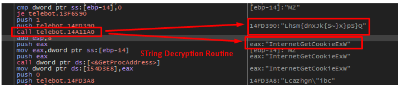
Figure 6: String Decryption Routine
