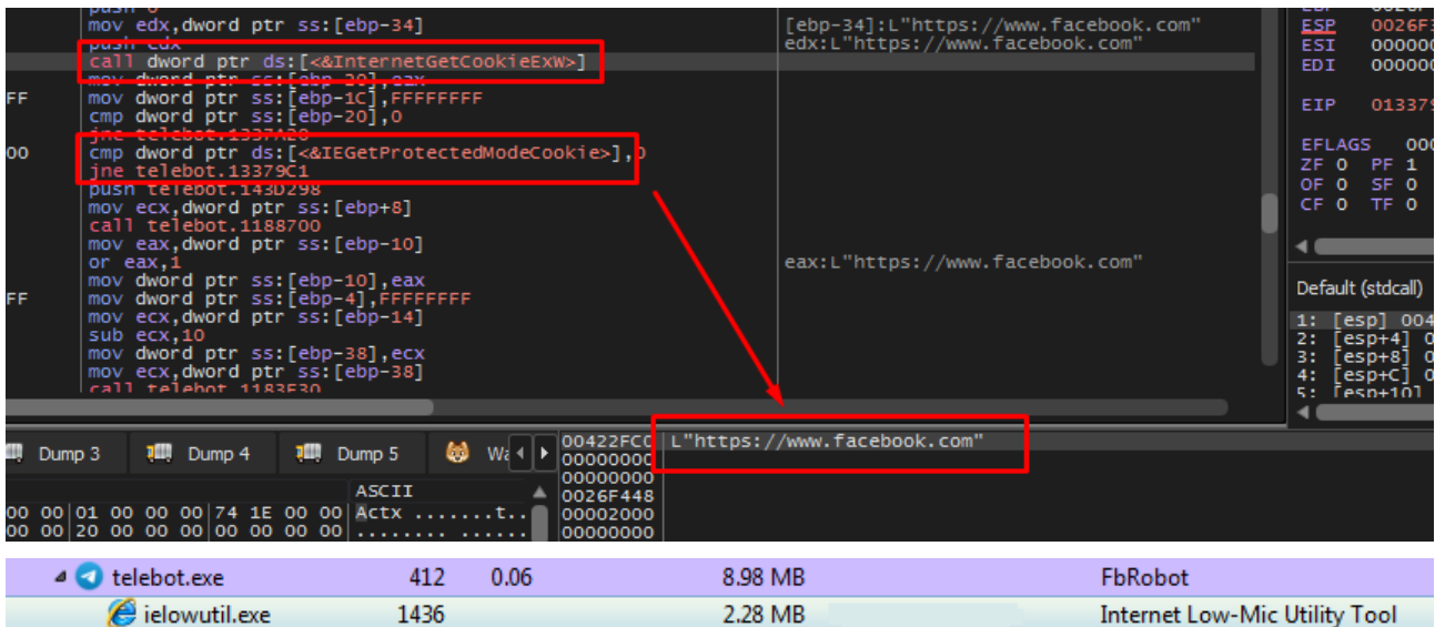
Figure 21: Execution of InternetGetCookieExW & IEGet ProtectedMode Cookie to steal cookies from the Internet Explorer browser
