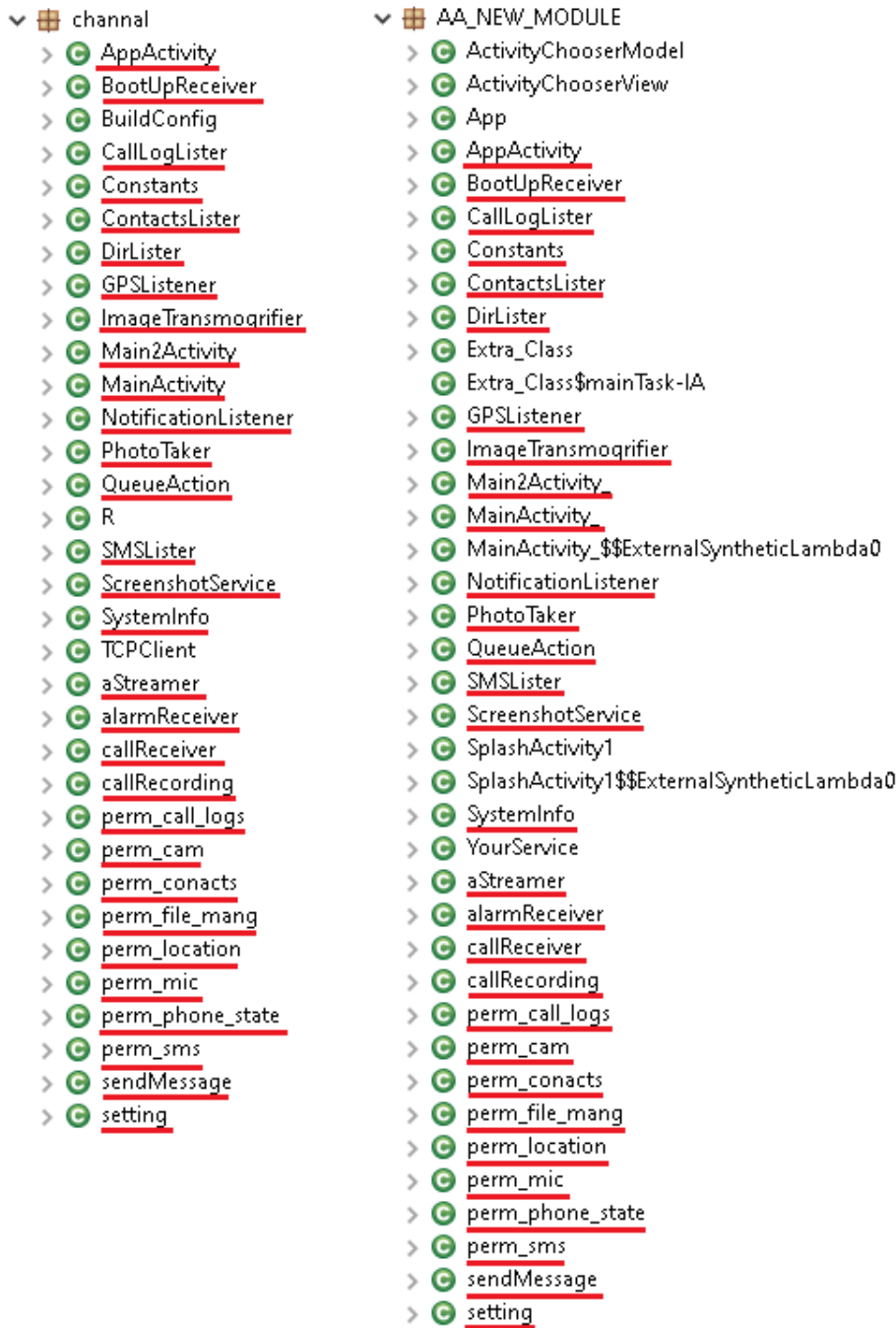
Figure 3. Malicious class name comparison of older CapraRAT (left) and more recent version (right)
