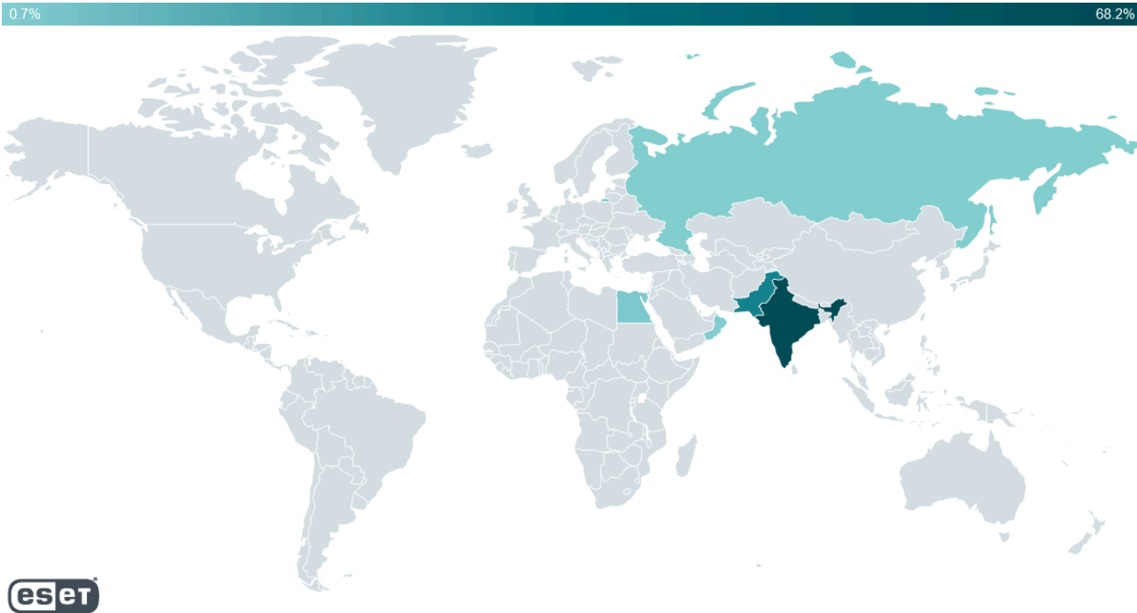
Figure 4. Victim distribution
