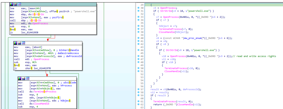
Figure 11: The payload enumerates for PowerShell process
