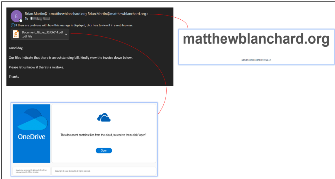
Figure 1: Phishing email
