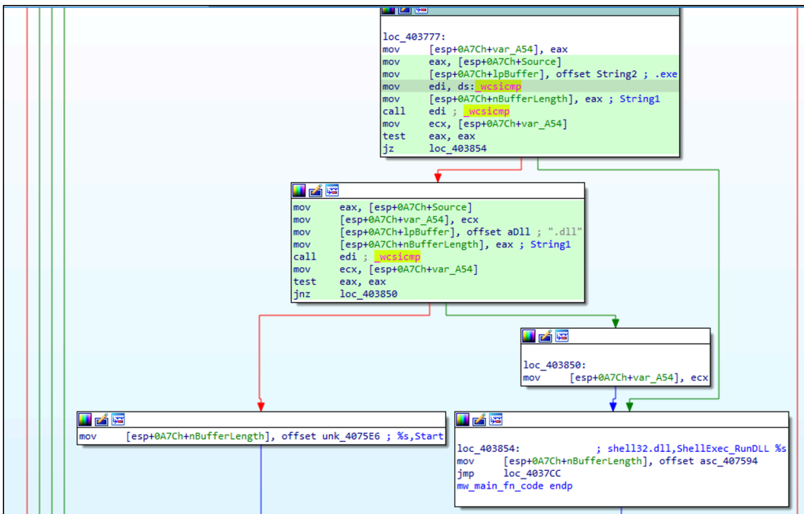
Figure 29: Extension check and execute the commands accordingly
