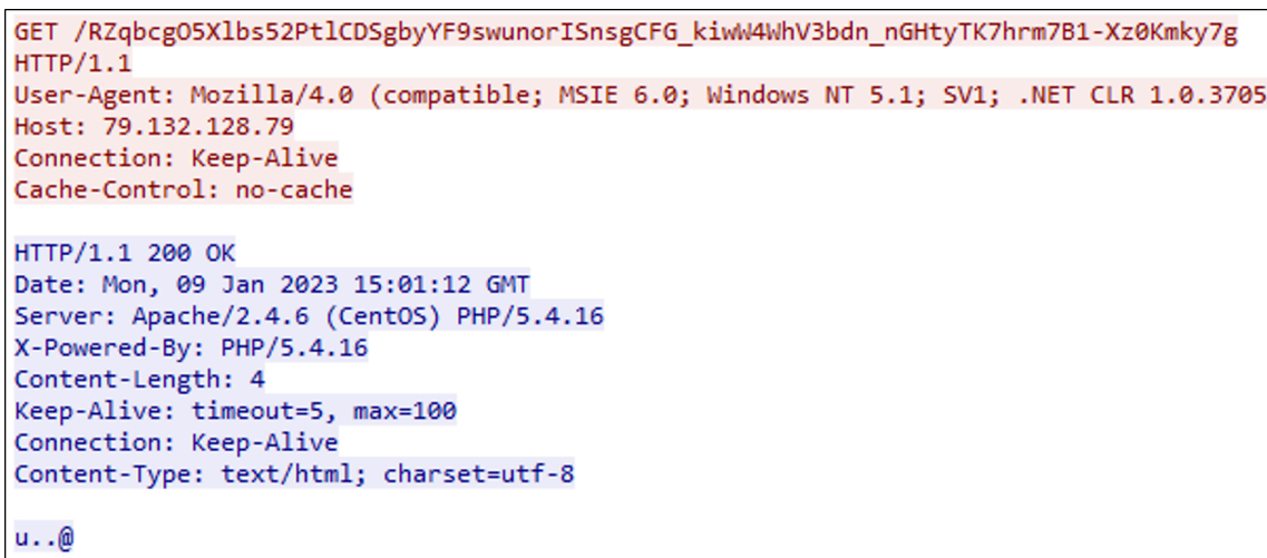
Figure 23: GET request within the pcap data
