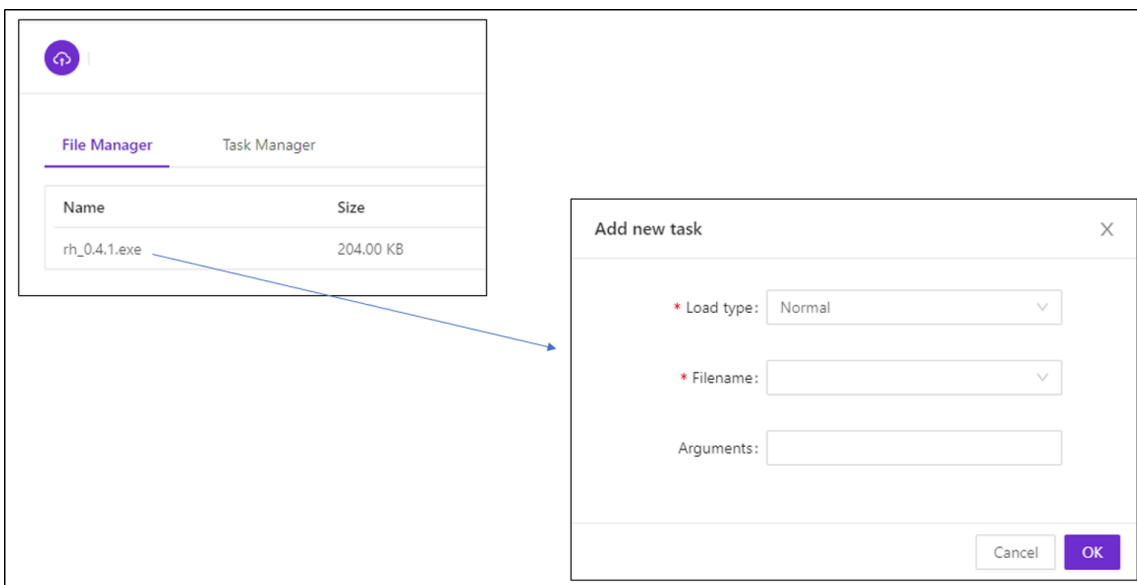
Figure 40: Task configuration
