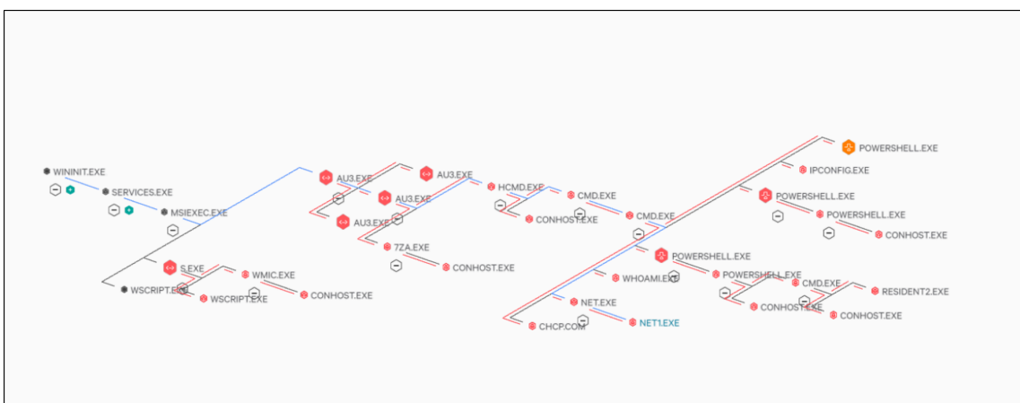
Figure 17: Infection chain (1)
