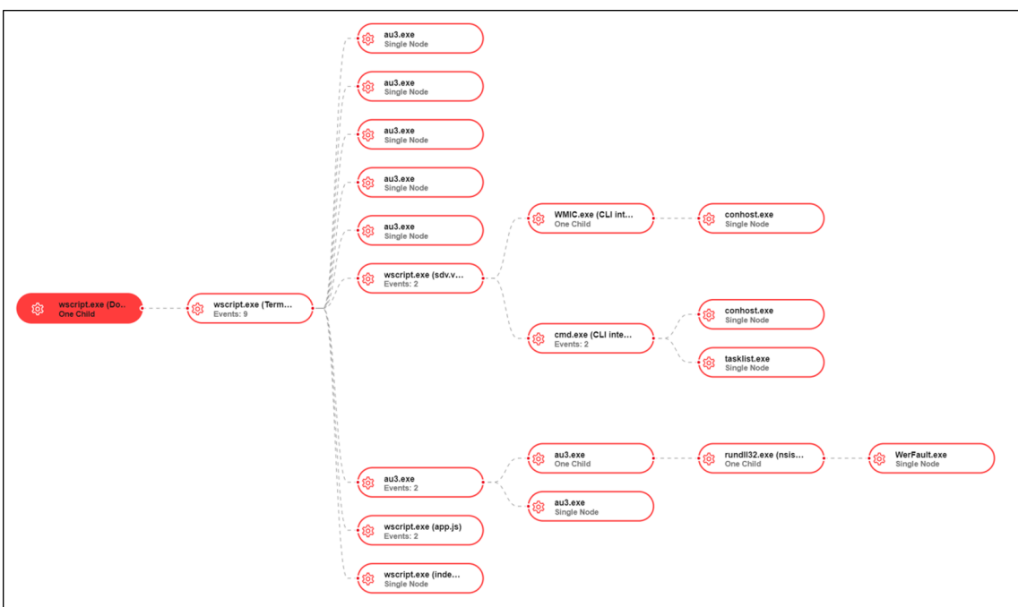
Figure 32: Infection chain (2)
