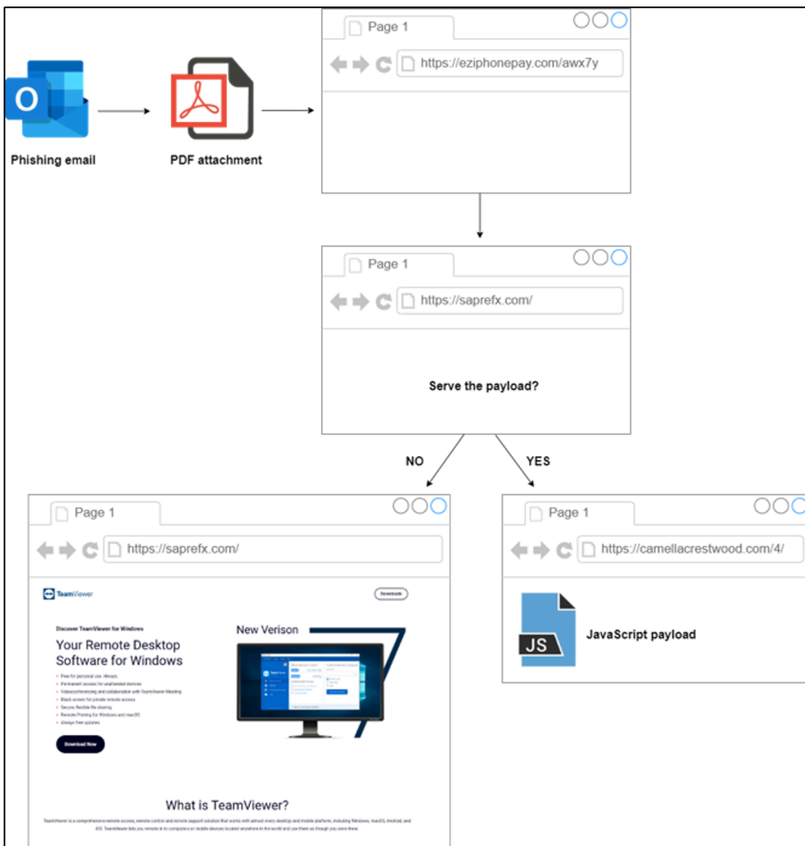
Figure 2: The redirect chain
