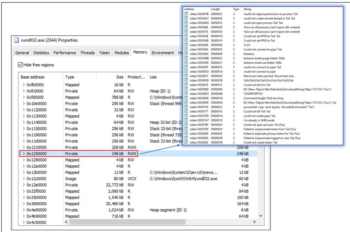
Figure 16: Cobalt Strike payload loaded into memory
