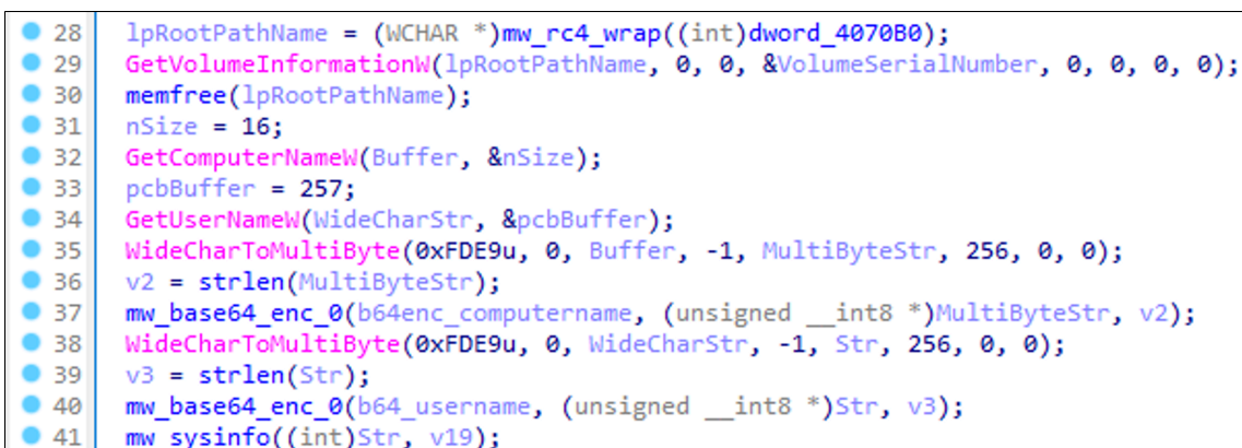
Figure 24: Retrieving the data and base64-encode them
