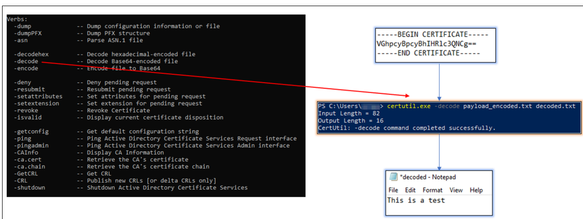
Figure 30: Example of how attacker(s) can abuse certutil.exe
