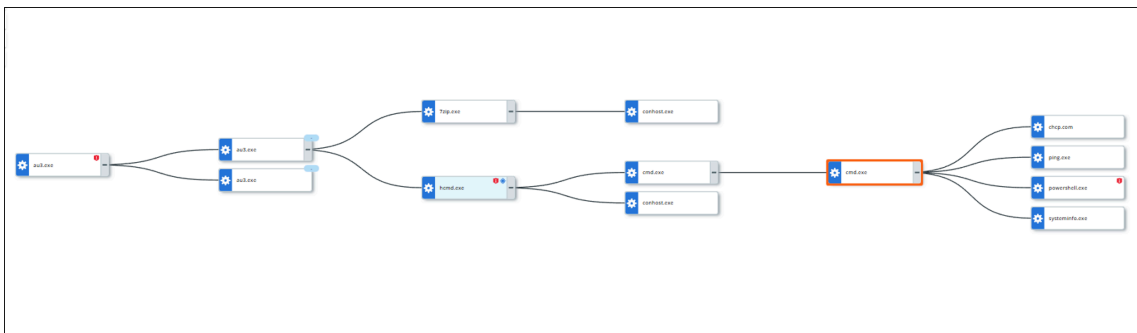
Figure 44: Infection chain (3)
