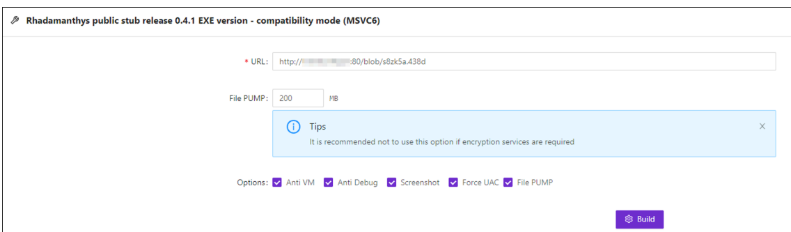
Figure 42: Build section
