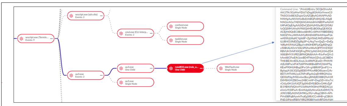
Figure 35: Stealer execution
