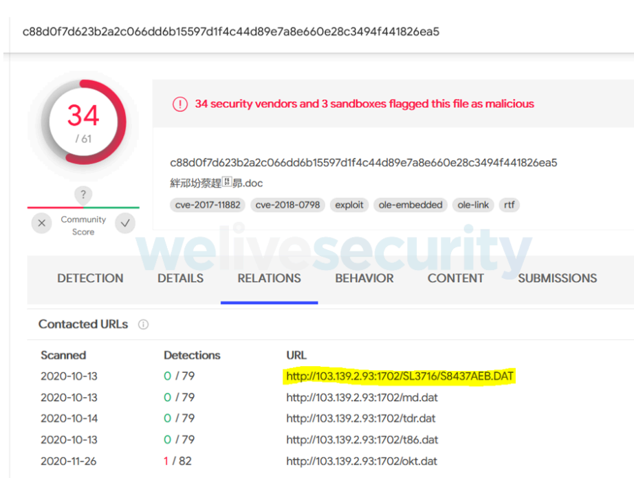
Figure 5. URL requests seen by the VirusTotal sandbox during execution of the malicious RTF document
