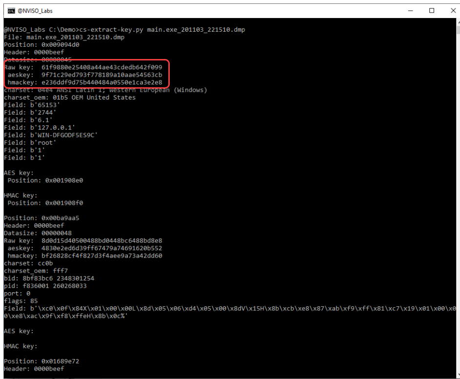
Figure 2: extracted and decoded metadata
