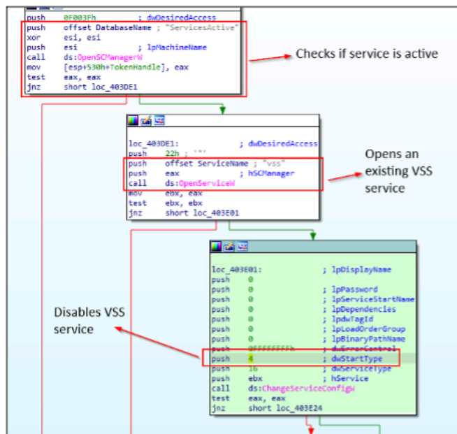
Exhibit 8: Disabling Volume Shadow Copy Service (VSS)
