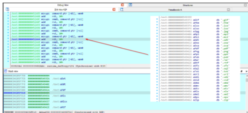
Exhibit 13: Populating the extensions from memory
