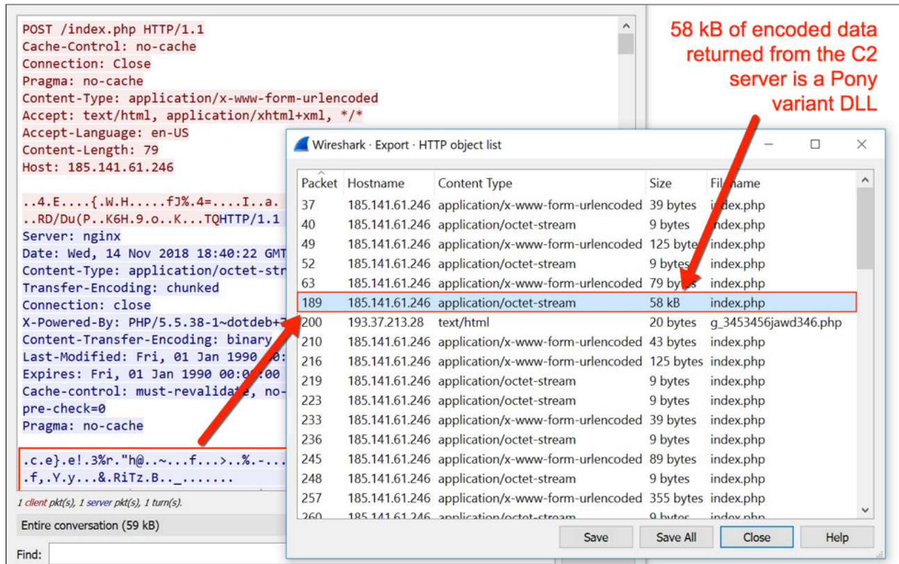
Figure 11: Using Wireshark to find 58 kB of encoded data returned from the C2 server at 185.141.61[.]246.
