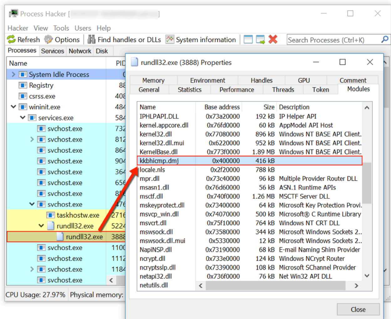
Figure 7: Example of a Redaman DLL persistent through a scheduled task.
