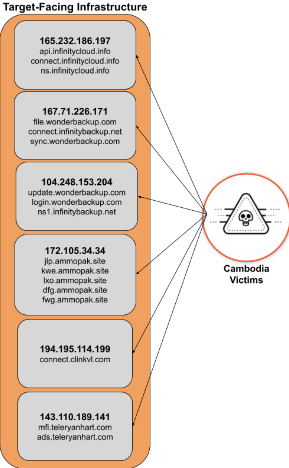
Figure 1. Infrastructure overview.
