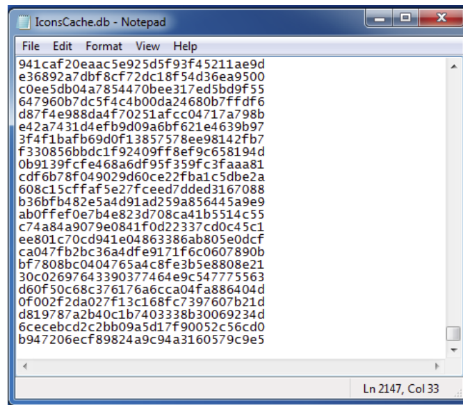
Figure 9. IconsCache.db contents.
