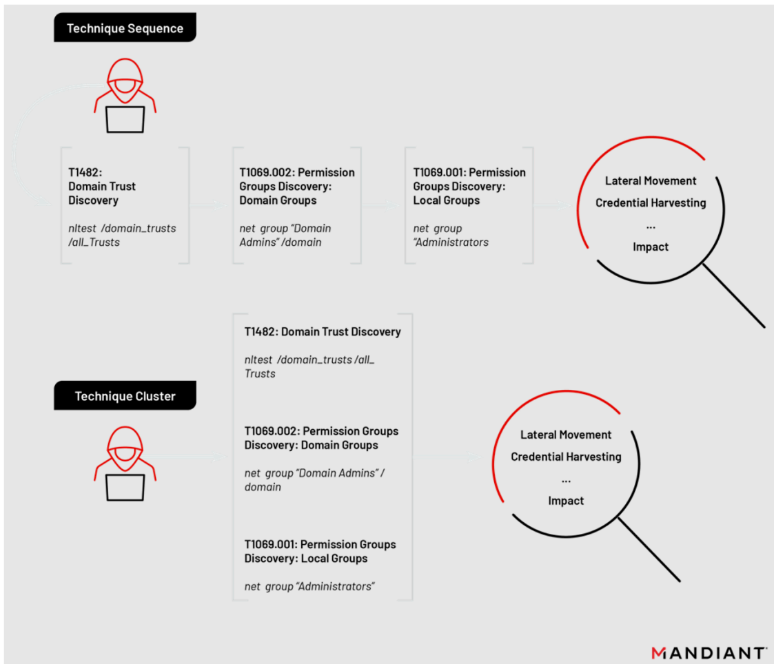
Figure 1: Visualization of technique sequencing and clustering concepts
