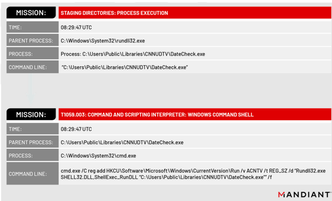
Figure 2: Technique sequence that led to UNC4191 detection
