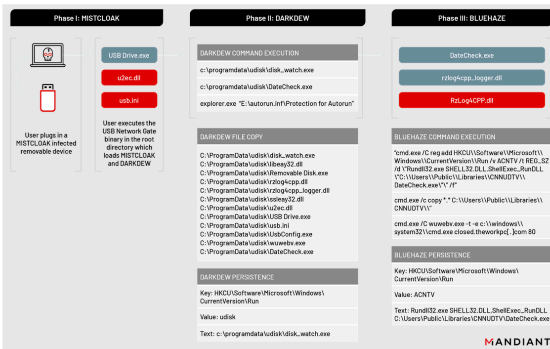
Figure 3: UNC4191 malware infection cycle
