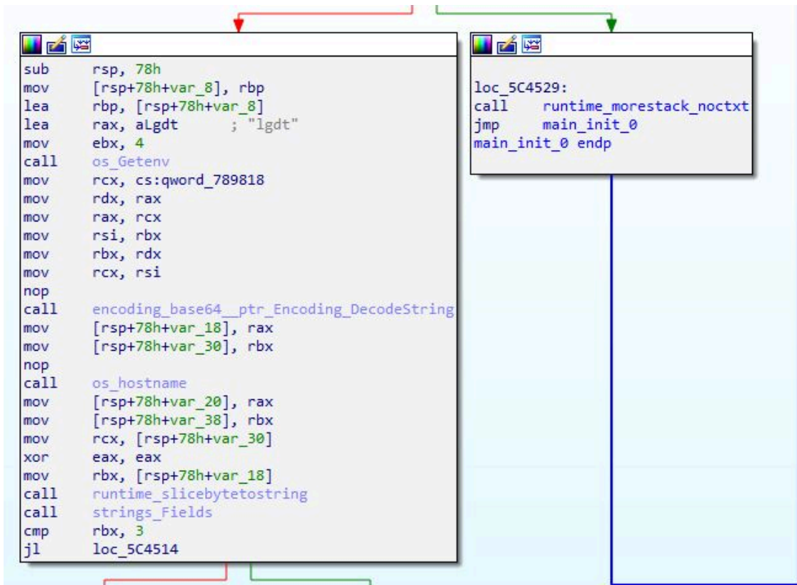
Figure 10. Routine that decrypts environment variables and uses them as configuration data
