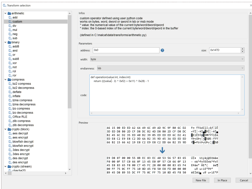
Figure 6: decrypting the shellcode
