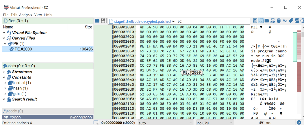
Figure 9: decrypted d54hdan9c9ebsx
