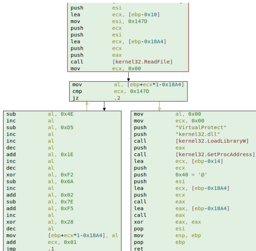
Figure 5: decryption loop in method sdvffryp
