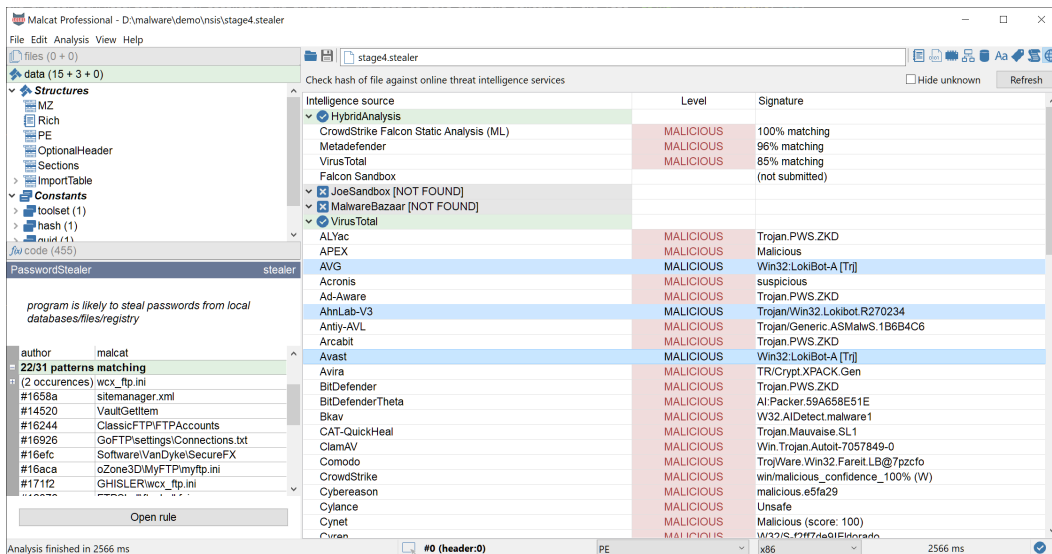
Figure 11: querying online intelligence
