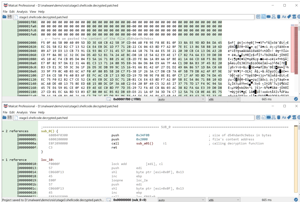
Figure 8: patching the shellcode
