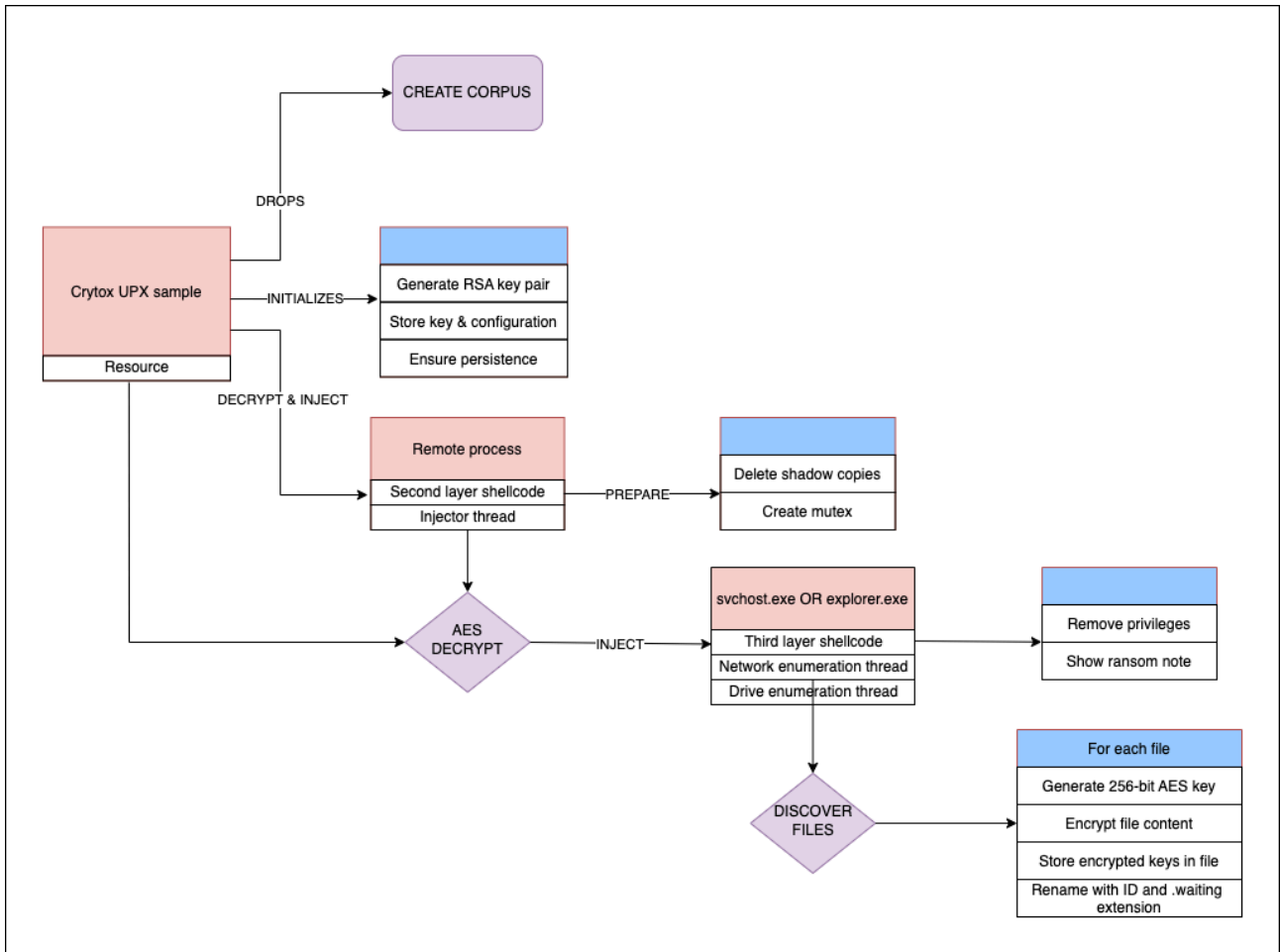
Figure 7. Process flowchart for Crytox encryption
