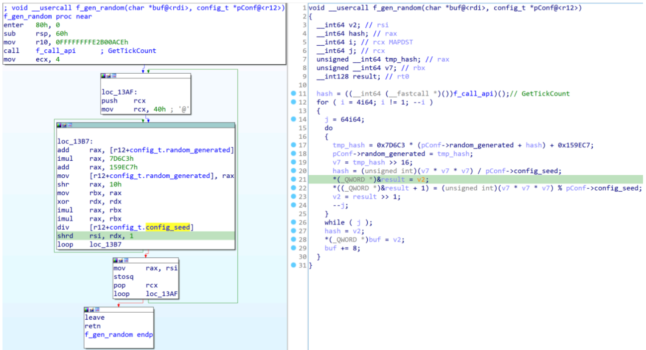
Figure 8. Cryptox key generation algorithm
