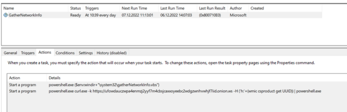
Figure 3: Trojanized GatherNetworkInfo task configuration
