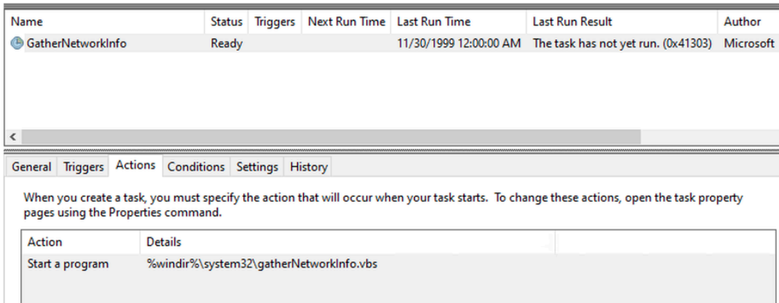
Figure 2: Legitimate GatherNetworkInfo task configuration
