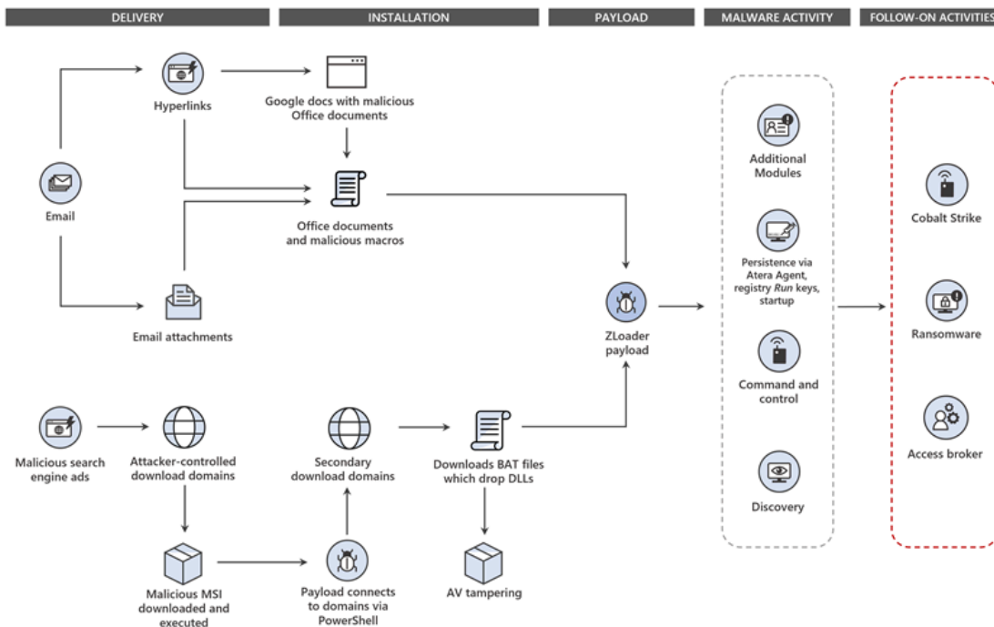
Figure 2. ZLoader attack flow diagram
