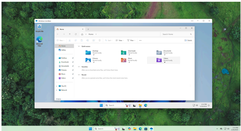
Figure 5. Windows Sandbox
