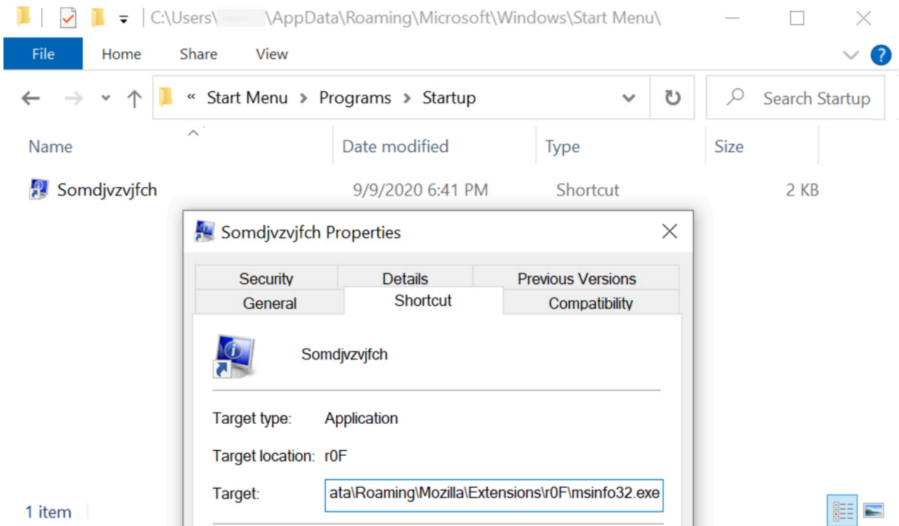
Shown above: Windows start menu shortcut also used to keep Dridex persistent on the same infected Windows host.
