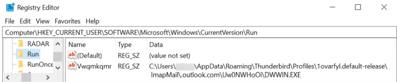
Shown above: Windows registry update used to keep Dridex persistent on an infected host.
