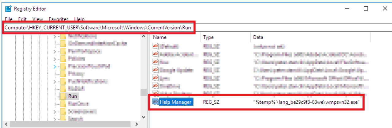
Figure 2: Registry entry used by the malware to gain persistence
