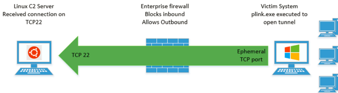
Figure 2: Example of successful RDP tunnel created using Plink
