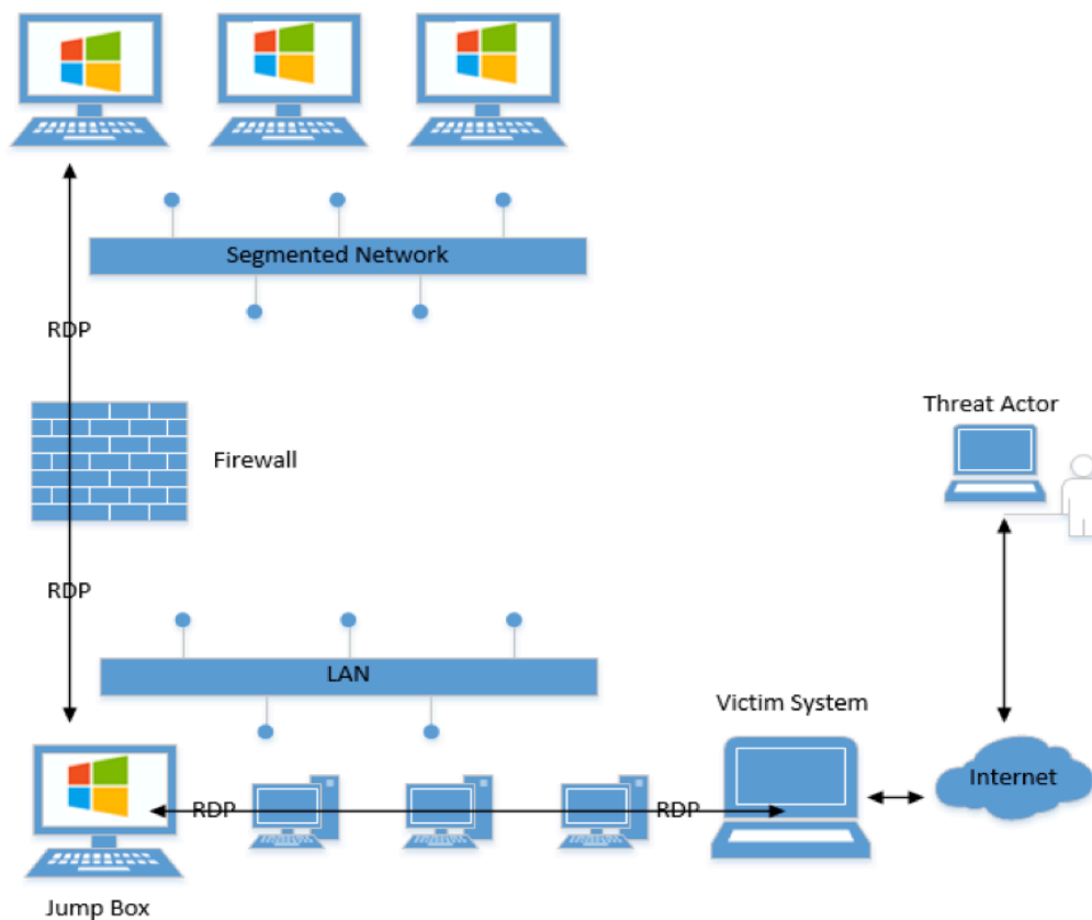
Figure 4: Lateral Movement via RDP using a jump box to a segmented network
