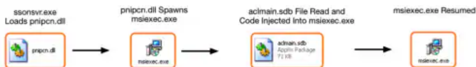
Figure 6 Sideload execution flow
