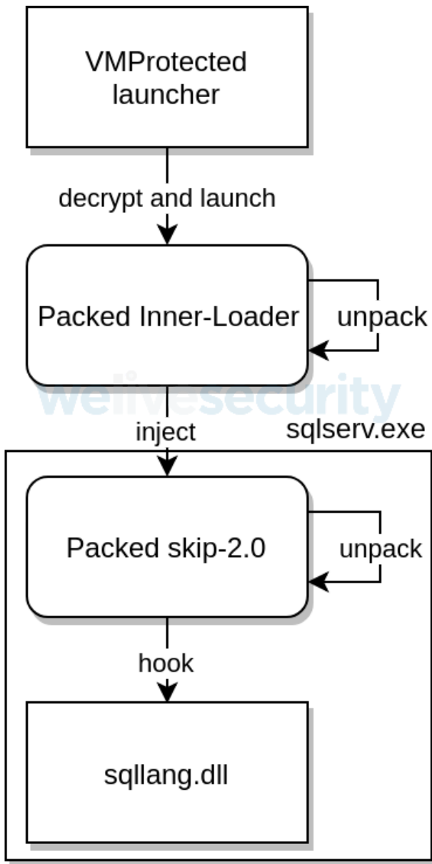
Figure 2. skip-2.0 unpacking and injection
