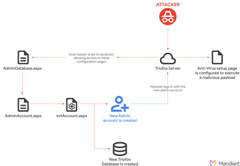
Figure 1: CVE-2025-12480 exploitation chain
