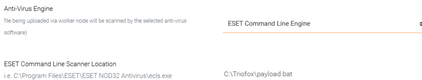
Figure 9: Anti-virus engine path set to a malicious batch script
