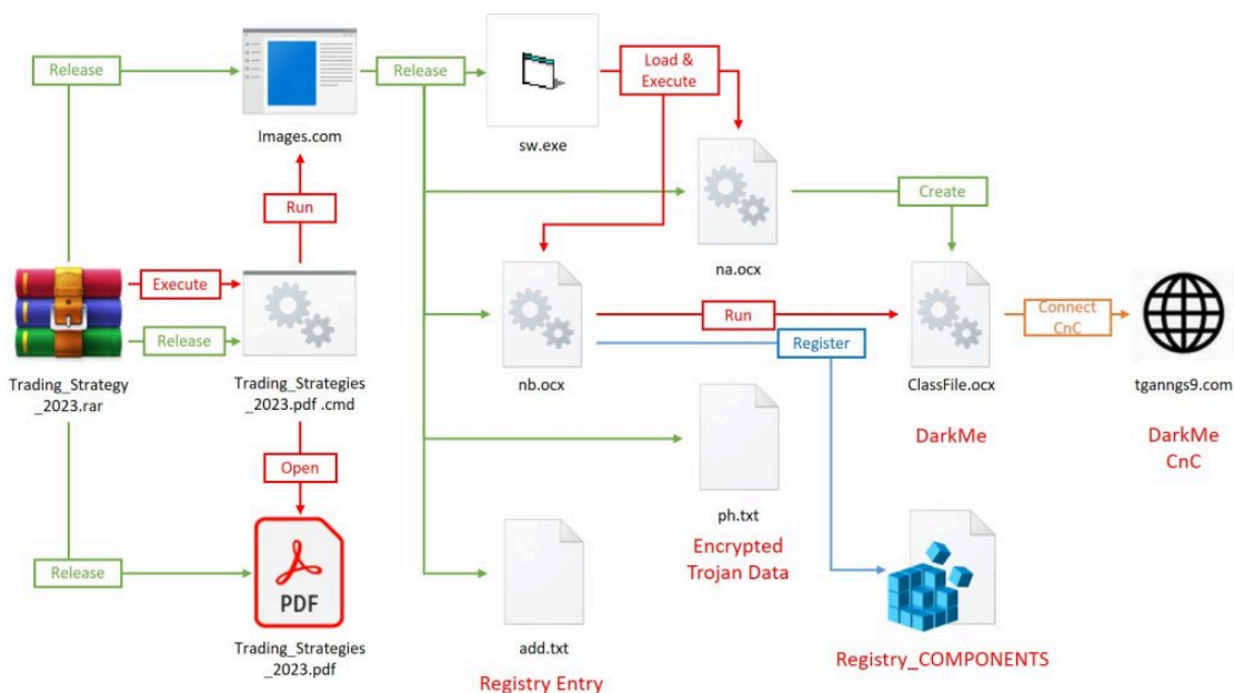
Figure 4.2 Main Attack Process of DarkCasino
