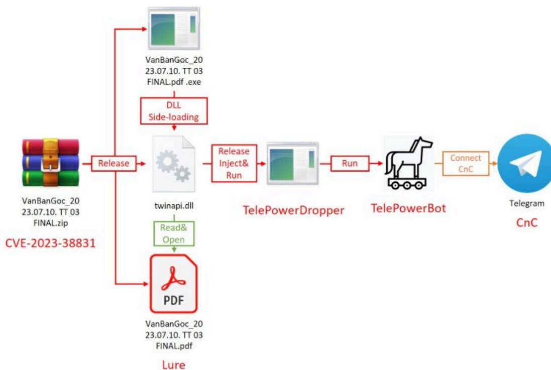
Figure 5.1 Main Attack Process of DarkPink
