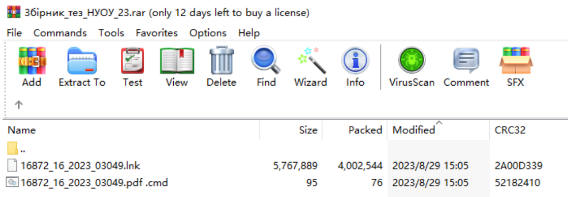
Figure 5.4 Vulnerability File Structure B Built by GhostWriter
