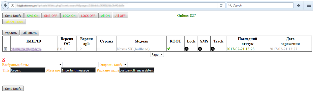
Figure 6 – C&C sending fake notification message to infected device
