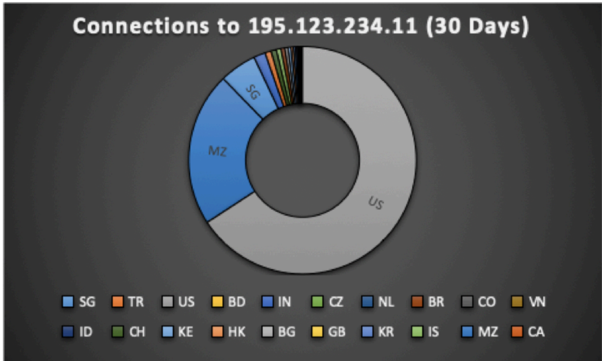
Figure 10. All traffic to 195[.]123.234.11 over a 30-day period
