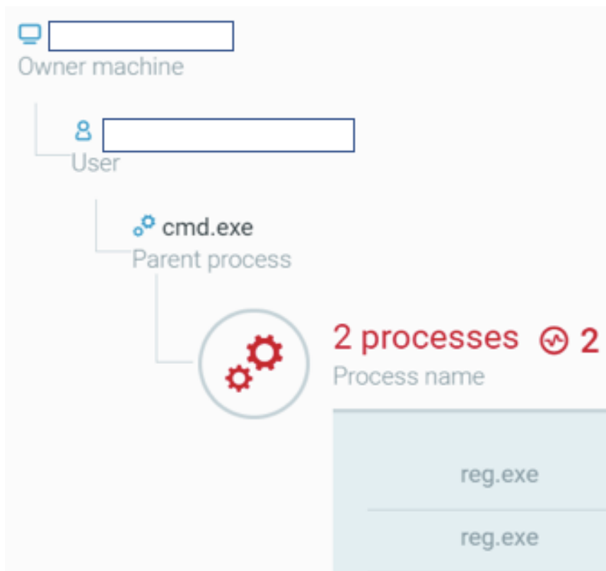
Reg.exe is being spawned from a
