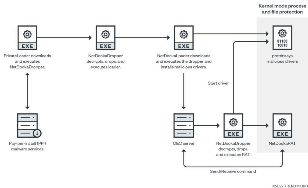
Figure 1. Infection chain of the attack
