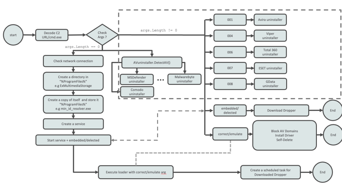
Figure 2. NetDookaLoader flow chart (Click to enlarge)
