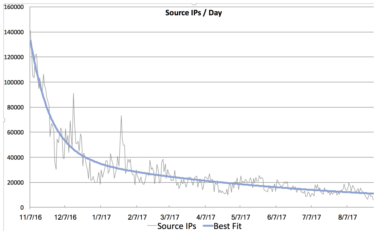
Figure 2: Decay of port 2323 scans and best fit.
