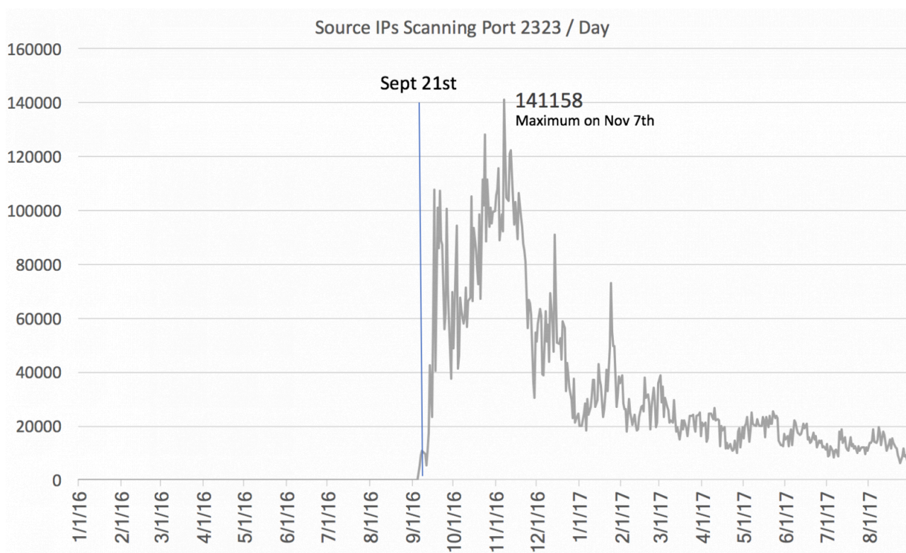
Figure 1: Port 2323 Scanning for 2016.
