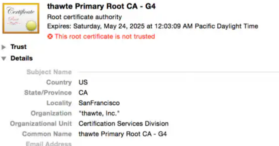
Figure 3: Fake “thawte, Inc.” Root Certificate installed by Retefe.
