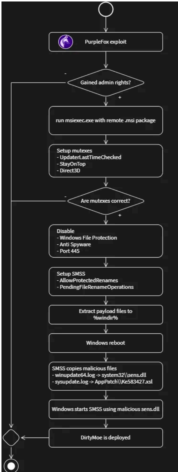
Figure 2. DirtyMoe deployment workflow
