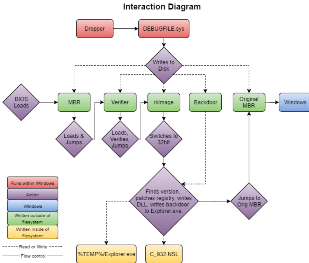
Figure 9: Diagram showing the out-of-OS boot process.
