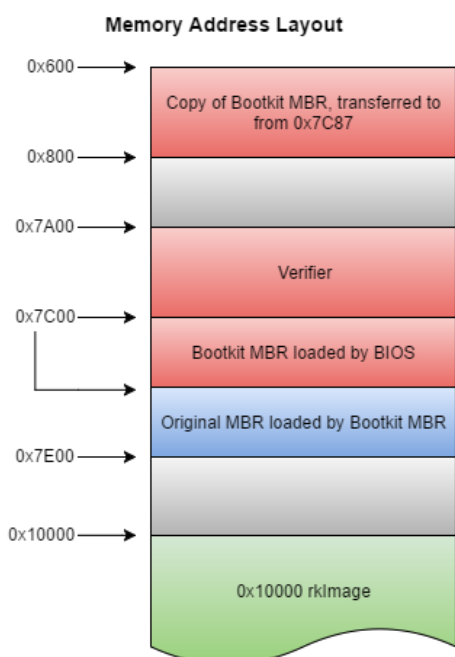
Figure 7: Address layout of memory loaded before rklImage
