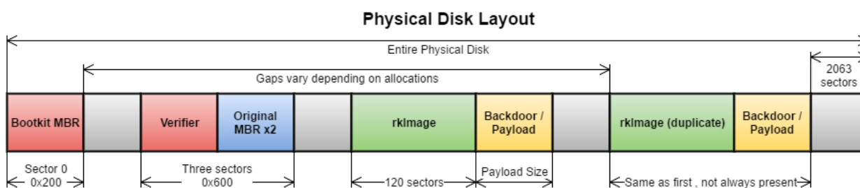
Figure 5: Physical Disk Layout written by DEBUGFILE.sys
