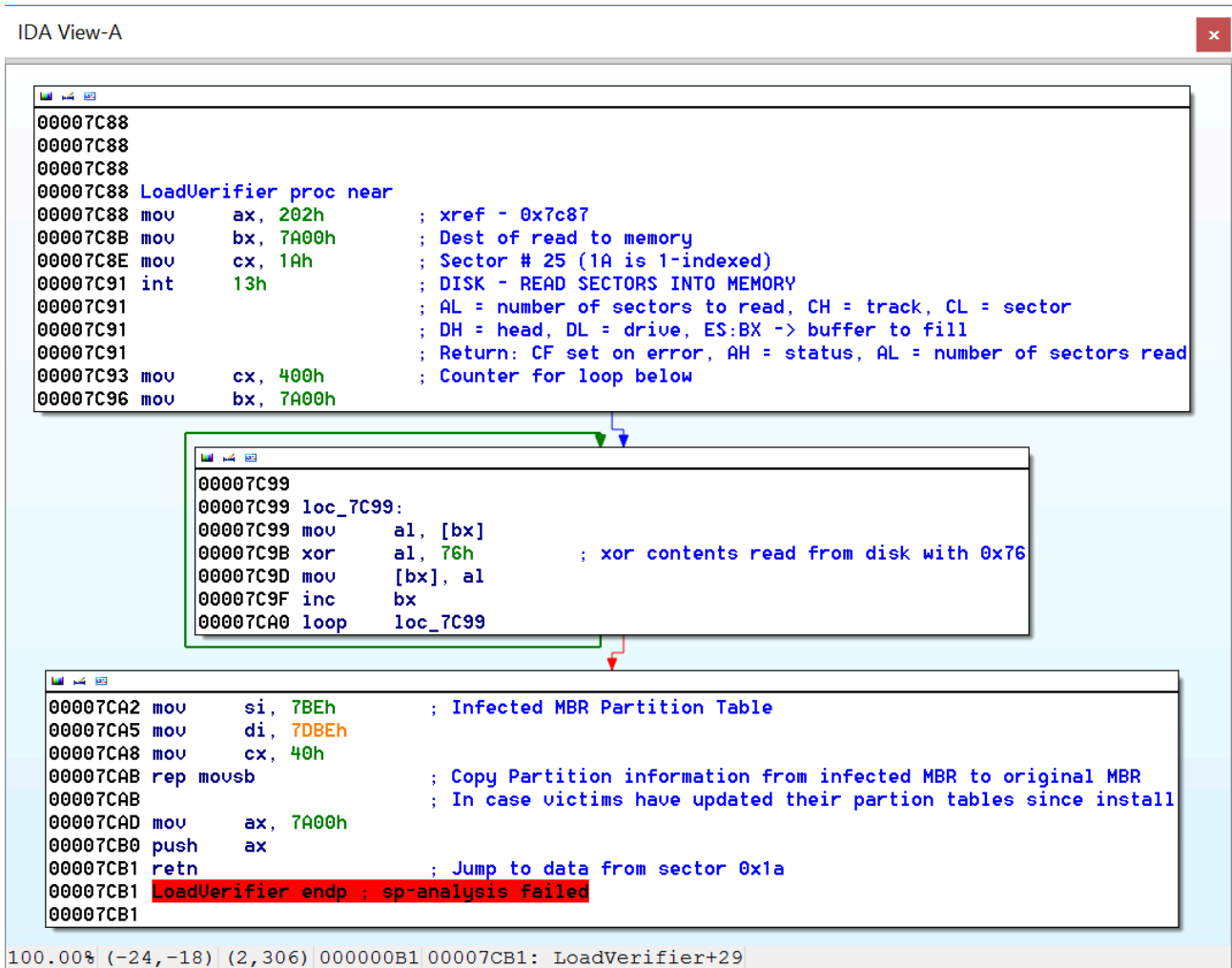
Figure 8: Infected MBR code to load, decrypt verifier
