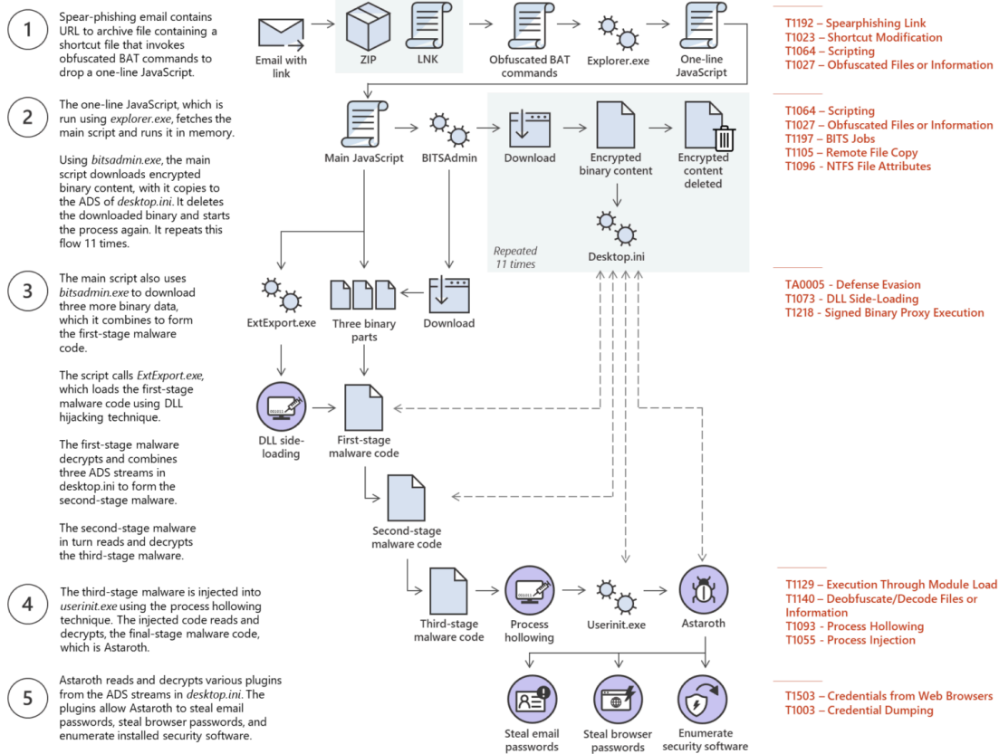
Figure 2. Astaroth attack chain 2020
