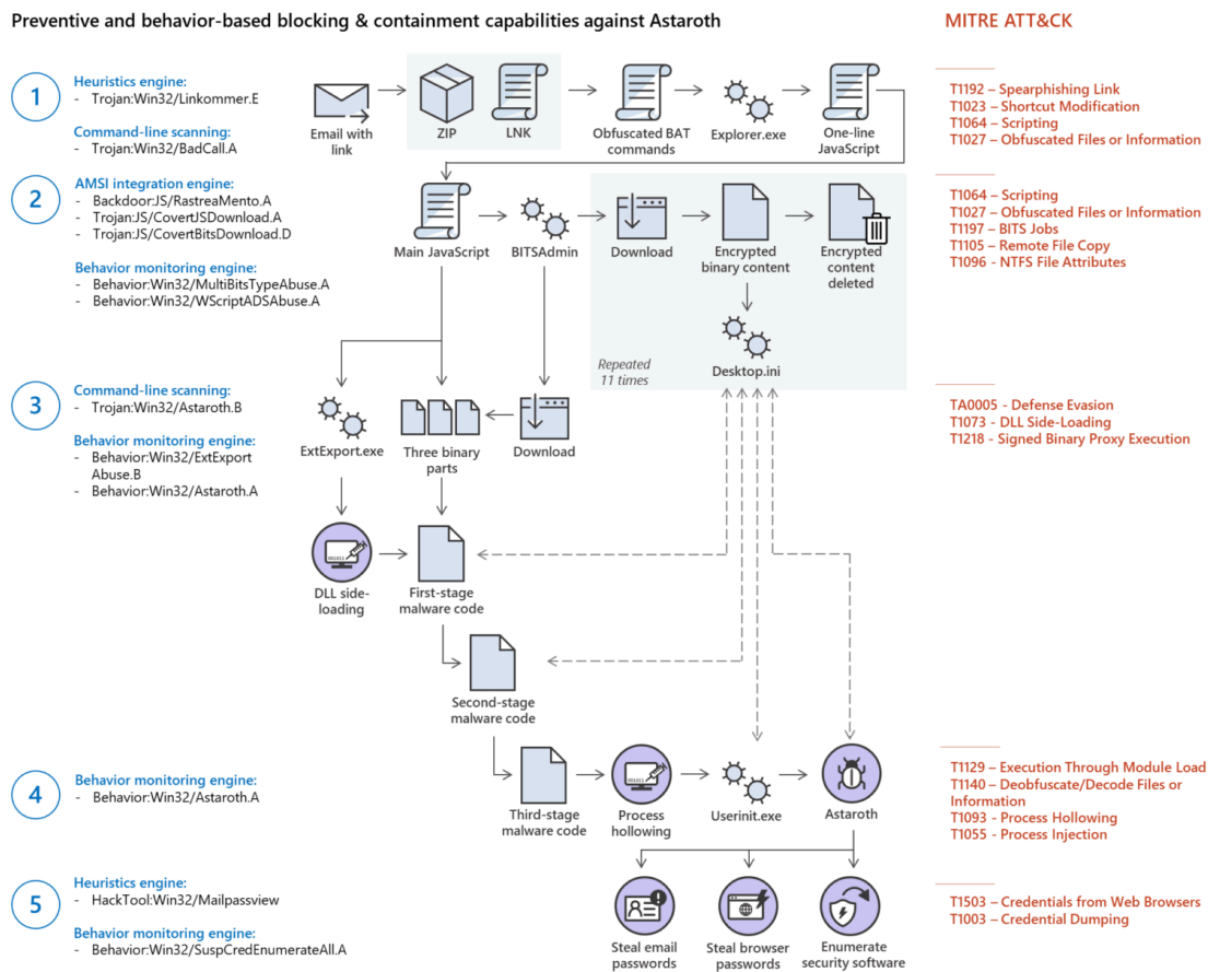
Figure 5. Preventive and behavior-based blocking & containment protections against Astaroth
