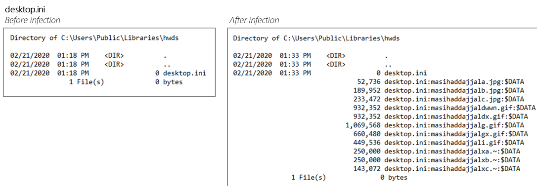
Figure 3. Desktop.ini before and after infection
