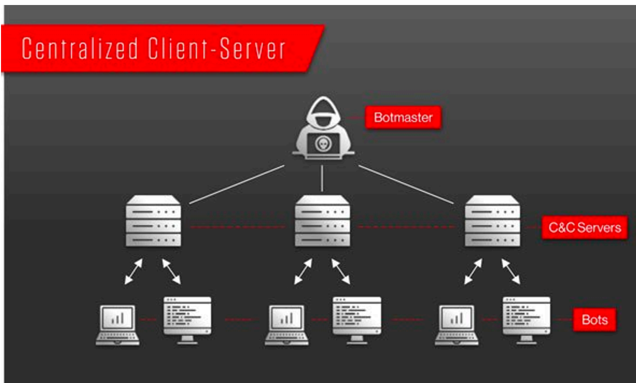
Figure 2. Example of Centralized Client-Server botnet infrastructure
