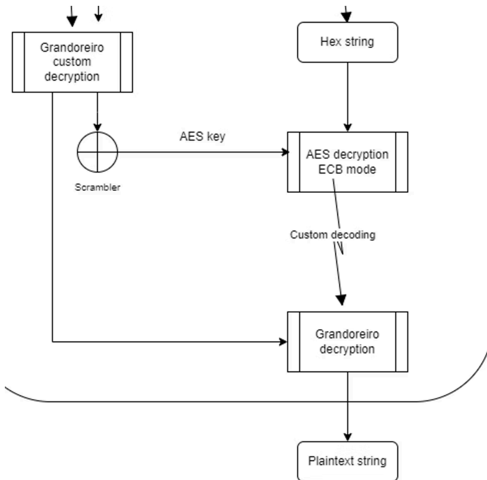
Fig 15: Grandoreiro banking trojan string decryption
