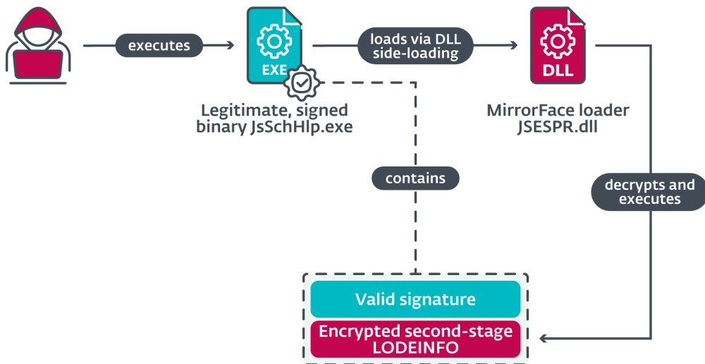
Figure 11. Execution flow of second-stage LODEINFO
