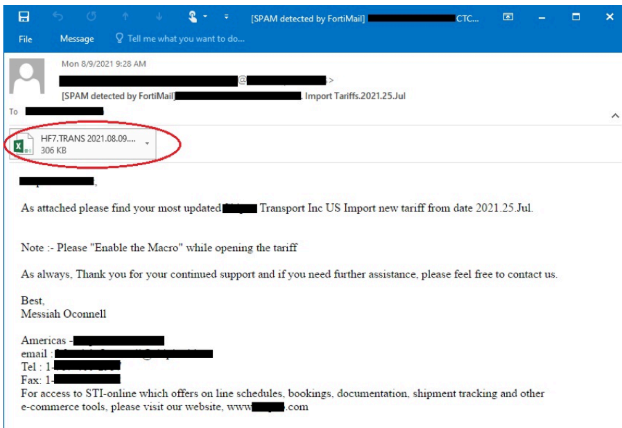
Figure 1.1 – Text of a recently captured phishing email
