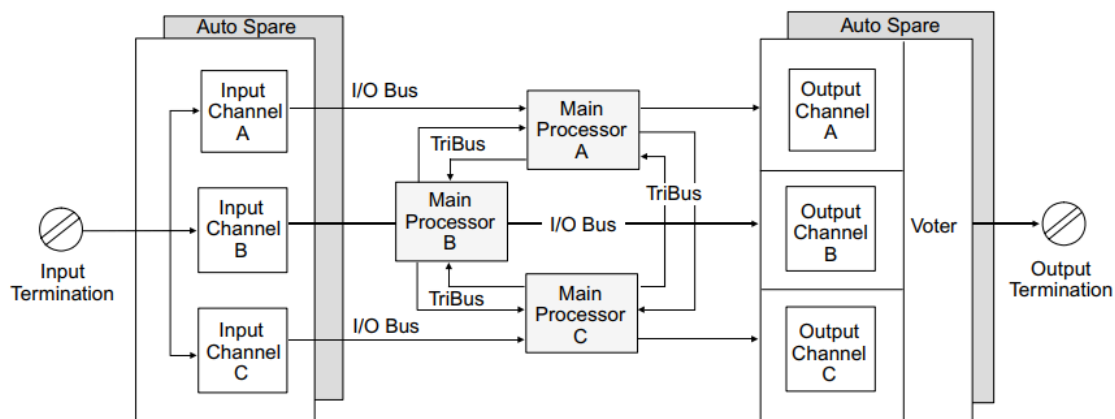
Figure 2 Triplicated Architecture of the Tricon Controller
