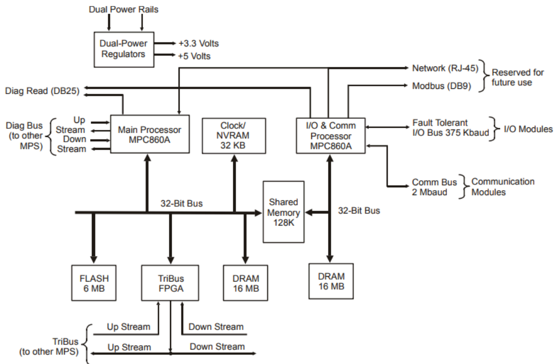
Figure 3 Architecture of a Model 3008 Main Processor
