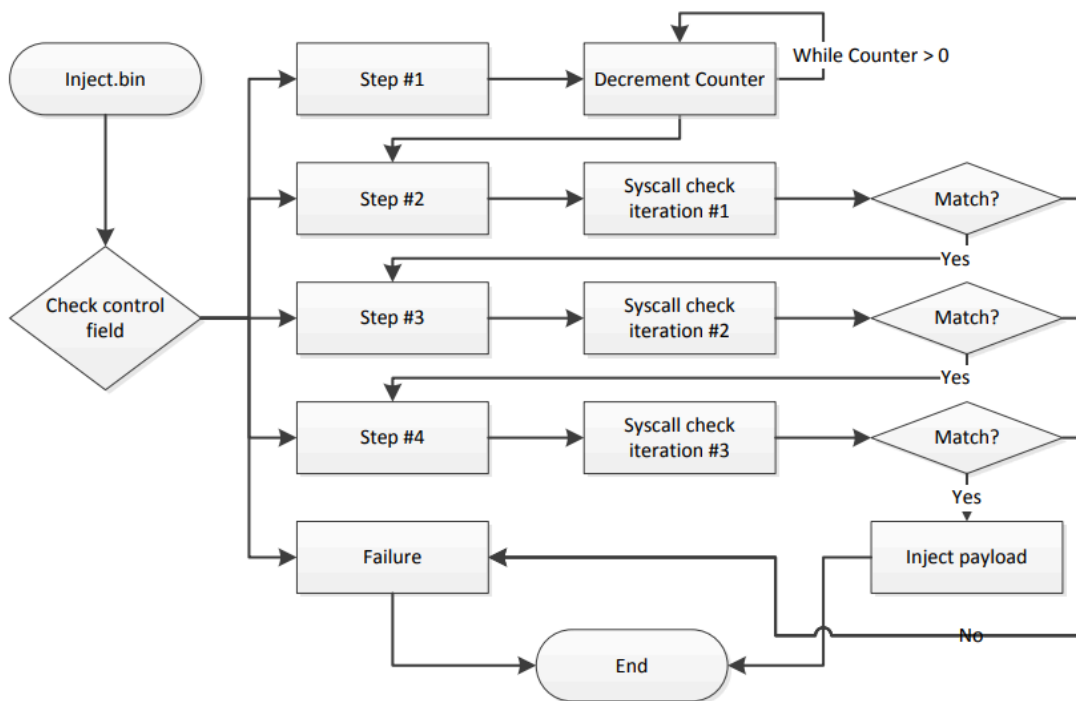
inject.bin control-flow ( source )
