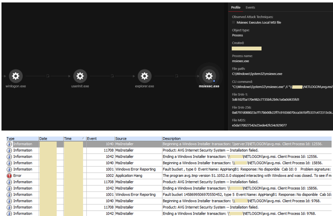
Figure 7. Manual installation of avg.msi failing
