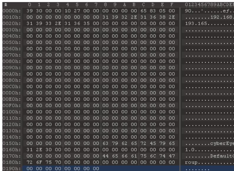
Figure 22. RtlShare backdoor configuration
