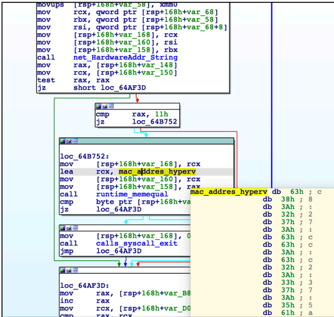
Figure 1: Mac address check
