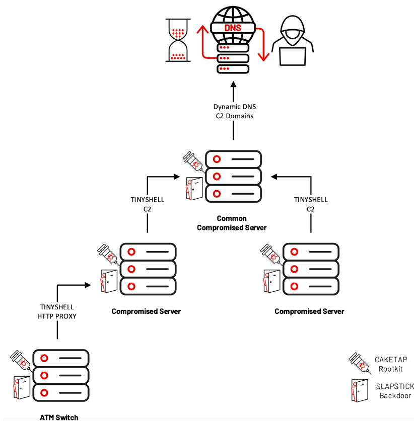
Figure 2: Example of TINY SHELL command and control used by UNC2891
