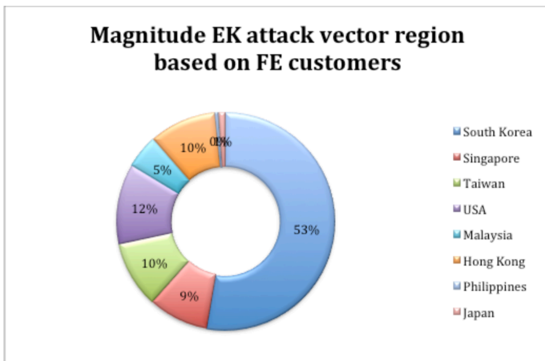
Figure 1: Magnitude EK distribution as seen in March 2017
