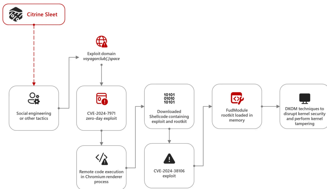
CVE-2024-7971 zero-day exploitation attack chain leading to FudModule rootkit
