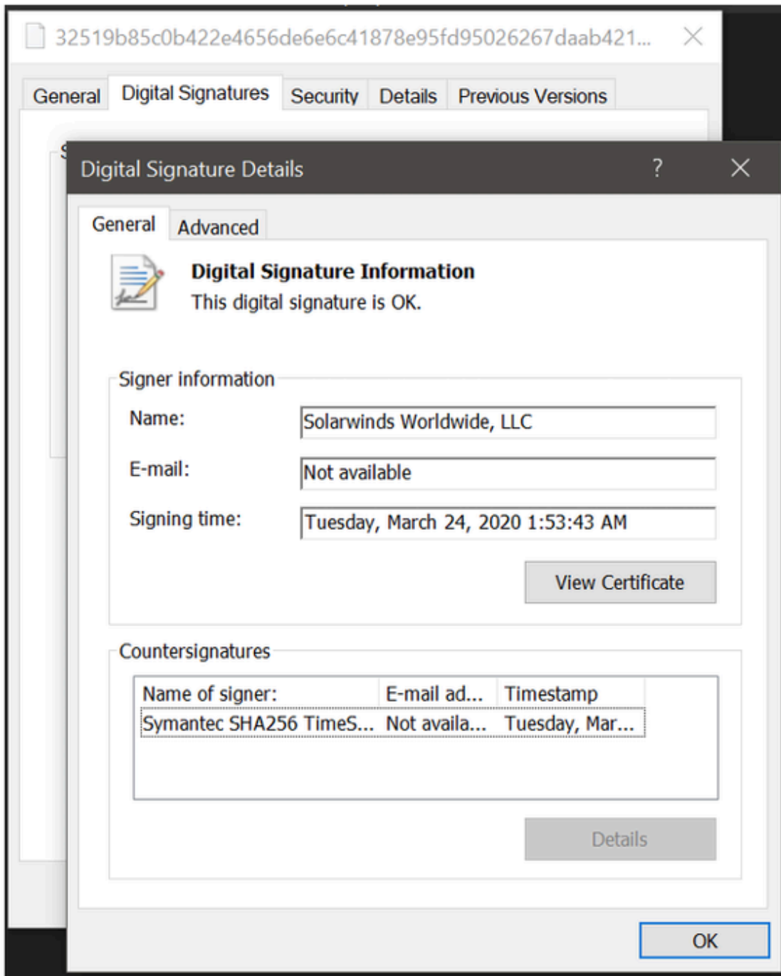
Figure 1: SolarWinds digital signature on software with backdoor
