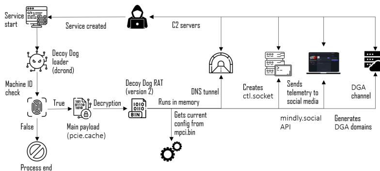
Figure 6. Decoy Dog flowchart
