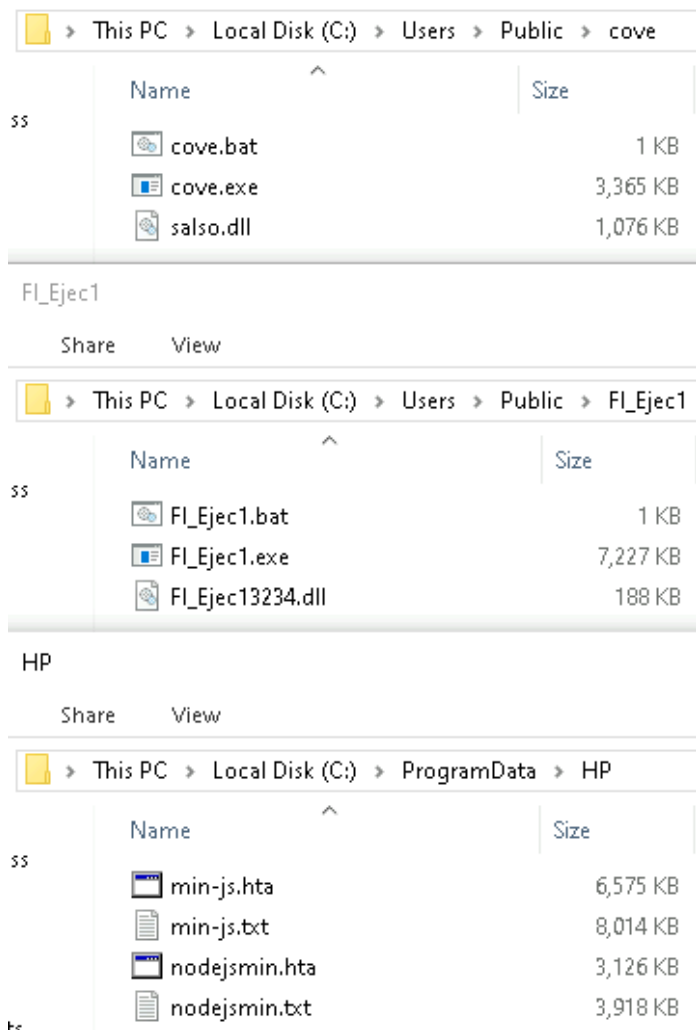
Fig. 2 – Files dropped in one of the campaigns
