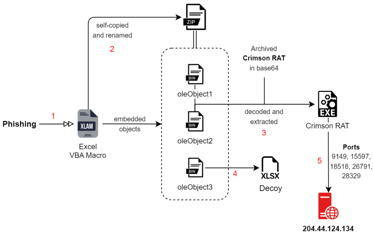
Fig. 10 – Infection Chain of APT36
