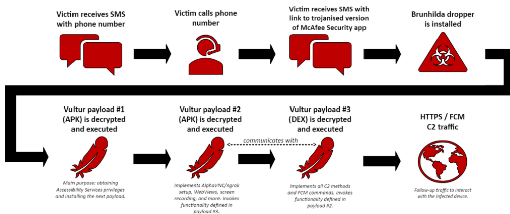
Figure 1: Visualisation of the complete infection chain. Note: communication with the C2 server occurs during every malware stage.
