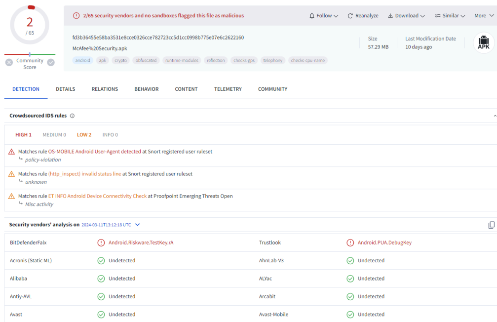
Figure 6: Brunhilda dropper’s detection rate on VirusTotal.
