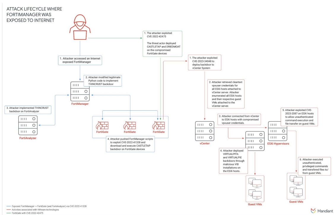
Figure 1: UNC3886 attack path diagram
