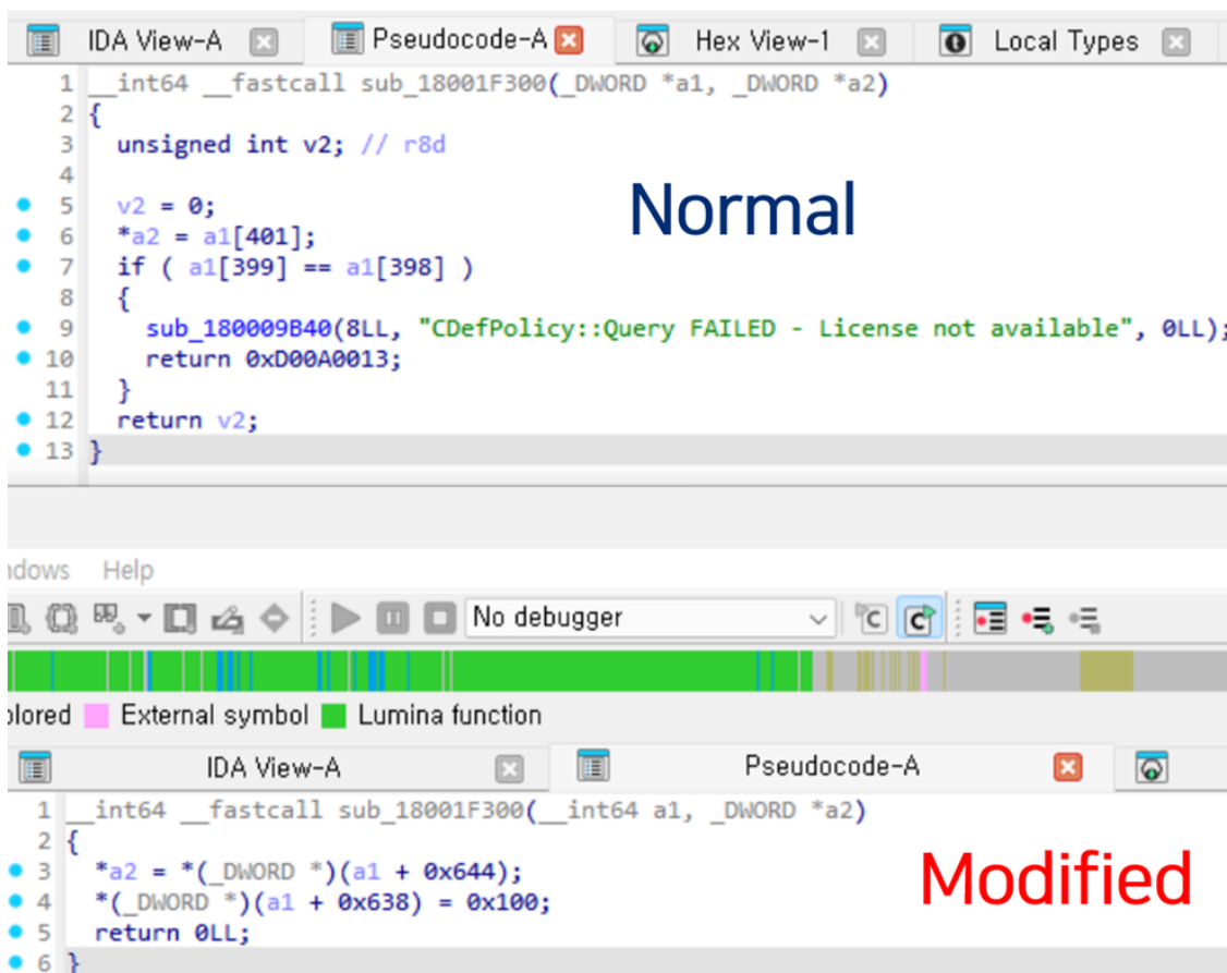
Figure 8. Comparison of the normal and patched modules (CDefPolicy::Query function)
