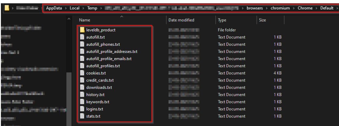
Figure 17 – Invicta Stealing the Browser Data from System
