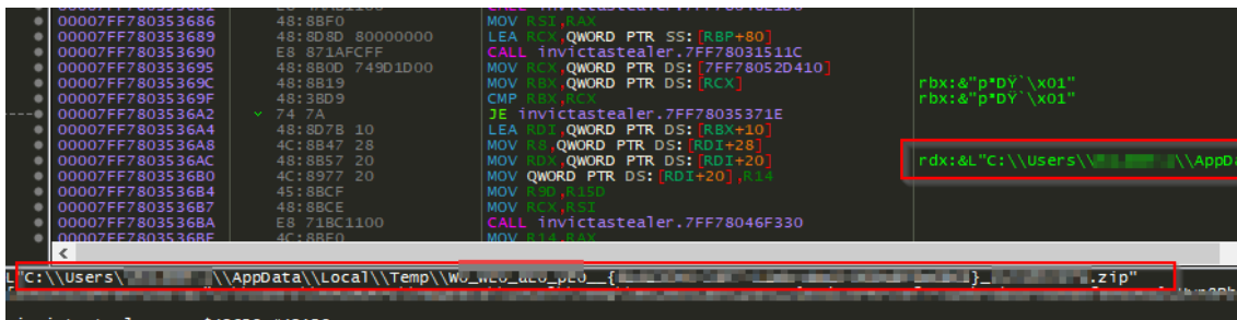
Figure 22 – Invicta Stealer Creating Zip File Containing Stolen Data
