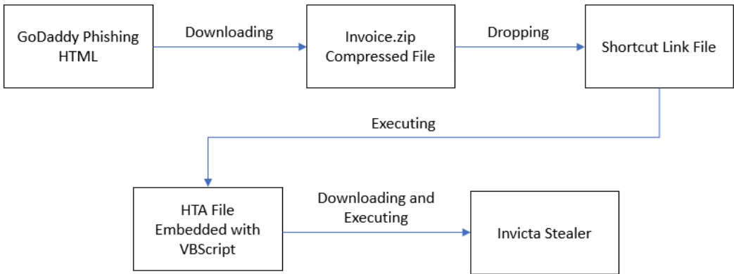
Figure 9 – Invicta Stealer Infection Chain
