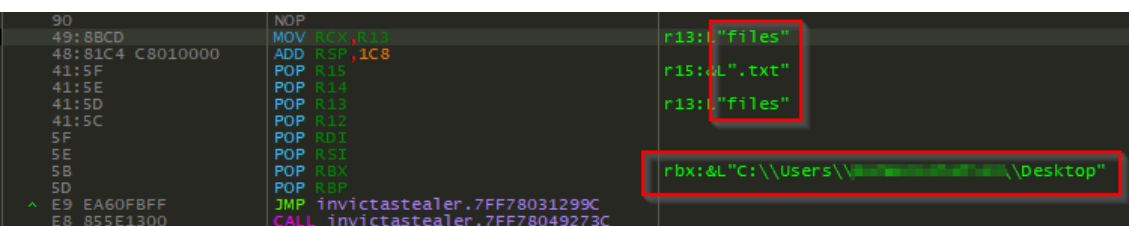
Figure 21 – Invicta Stealer Targeting the Files in the System
