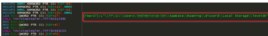
Figure 13 – Invicta Stealer Targeting Discord
