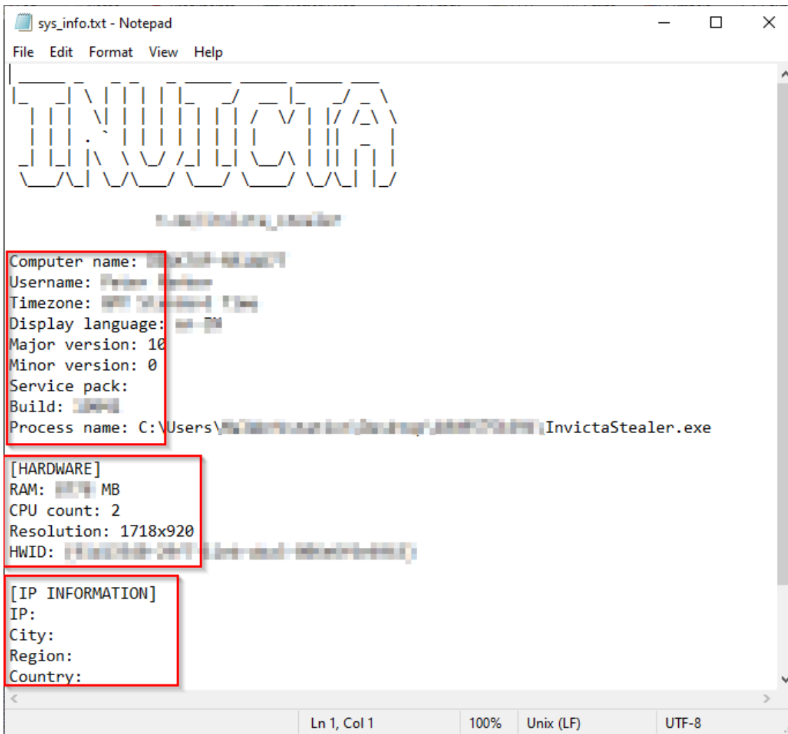
Figure 12 – sys_info.txt File Containing the System Details
