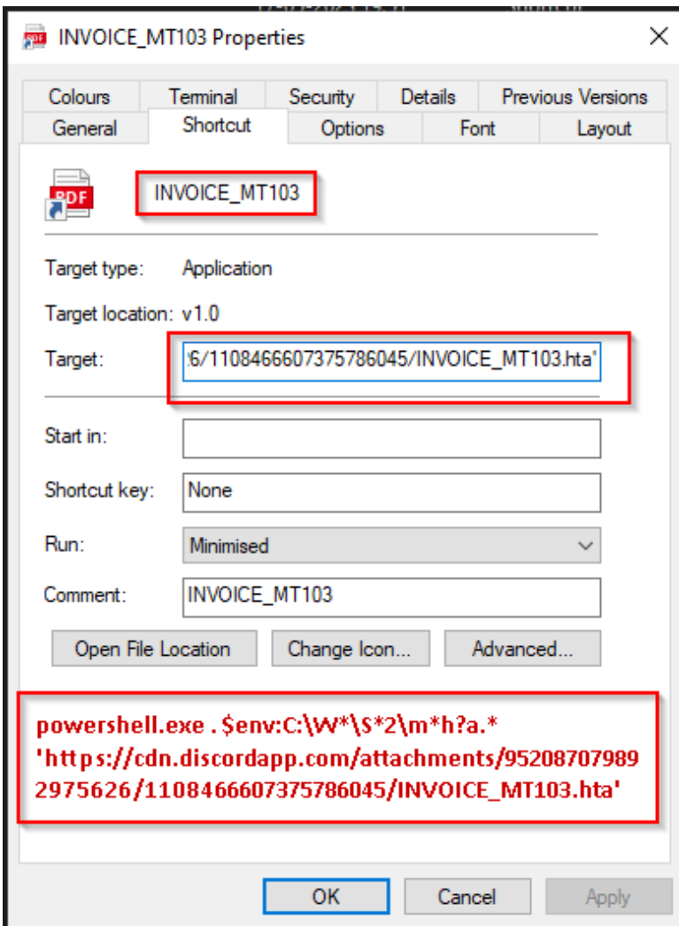
Figure 7 – Details of the Malicious Link File
