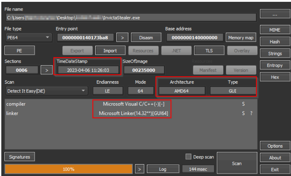
Figure 10 – Invicta Stealer File Details
